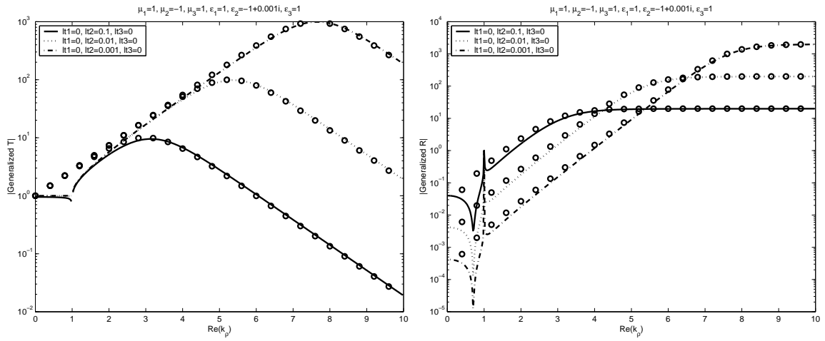
Figure 16: The magnitude of the LHM slab transmission coefficient (left) and reflection coefficient (right) along the real axis integration path for decreasing loss tangents. The circles are the asymptotic approximation to the formula for large k_\rho . Here, \omega = \mu_0 = \epsilon_0 = h = 1
