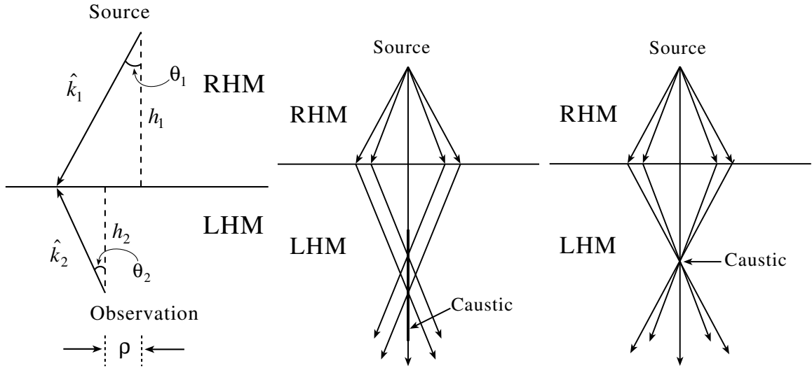
Figure 11: (Left) The parameters for the condition given by Equation (24) for focussing. The rays for the unmatched case (center) form a caustic along the vertical z axis while the rays for the matched case (right) form a caustic at the focal point.
