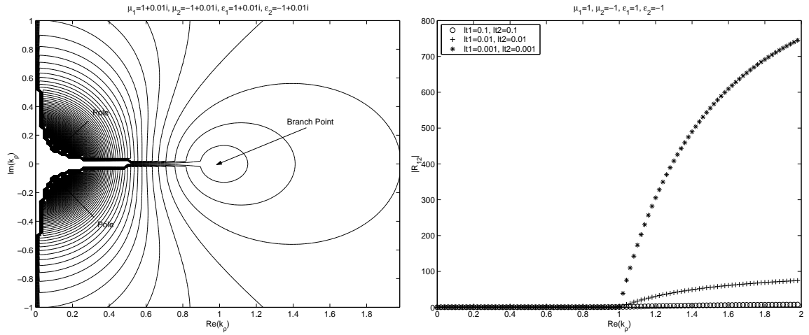
Figure 9: (Left) The contour plot of the magnitude of the reflection coefficient for a matched double negative material for the lower half space. Two poles are observed, and the two branch points almost coalesce into one branch point. (Right) Reflection coefficient plot along the real axes shows large values for evanescent spectrum (to the right of the branch point) for different loss tangents. \omega = \mu_0 = \epsilon_0 = 1 .
