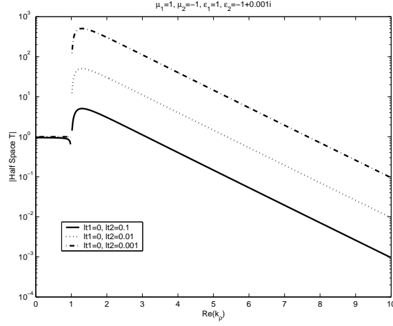
Figure 10: The transmitted field through a matched LHM half space at a distance h = 1 below the interface for different losses. \omega = \mu_0 = \epsilon_0 = 1 .
