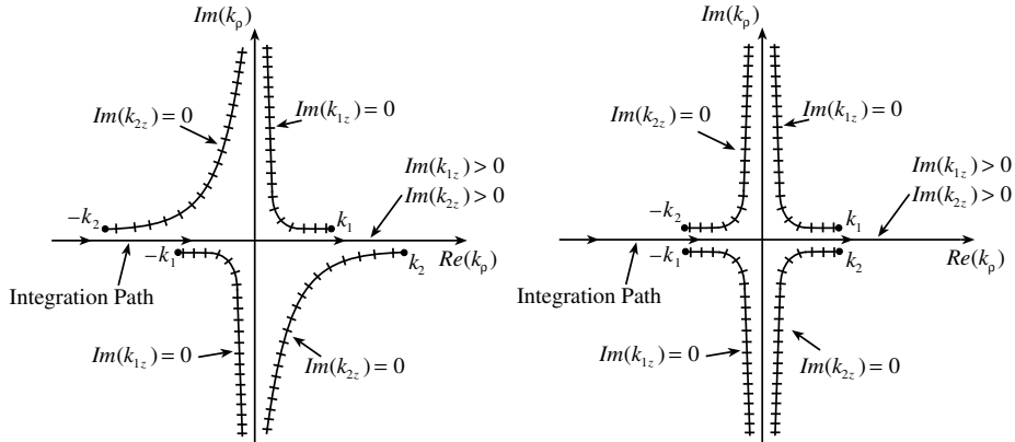
Figure 4: The branch cuts and Riemann sheets for a point source on top of the lossy RHM/LHM half spaces, (left) unmatched case and (right) matched case. \Re(k_{1z}) > 0 , \Re(k_{2z}) < 0 on the integration path. For 2D problems, the integration path is from -\infty to +\infty , while for 3D problems as in this paper, it is from 0 to +\infty .
