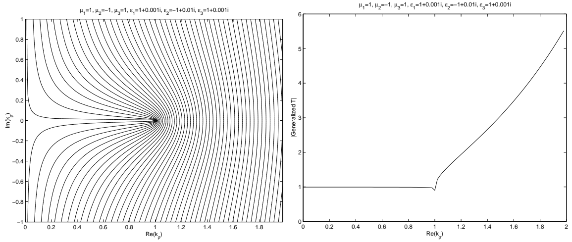
Figure 14: The contour plot of the magnitude of the LHM slab transmission coefficient (left) and the same coefficient along the real axis (right). Here, \omega = \mu_0 = \epsilon_0 = h = 1 .
