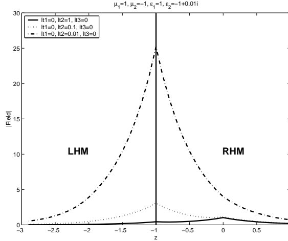
Figure 8: The total (incident and reflected) evanescent field for an interface with plasmon resonance. The lower the loss, the larger the reflected and transmitted field. The source at z = 0 generates the evanescent wave with unit amplitude and the interface is at z = -1 .
