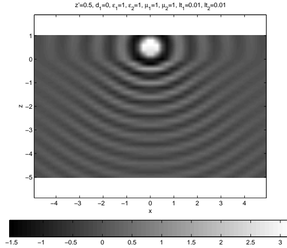
Figure 5: A point source at an ordinary RHM interface generates spherical and lateral waves as seen in this figure [24, p. 109]. x and z are in units of free space wavelengths.
