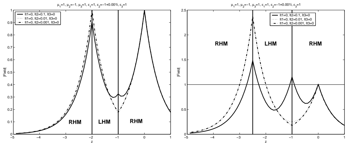
Figure 13: The propagation of the plane evanescent field from the source point at z = 0 into a thin LHM slab (left) and thick LHM slab (right).
