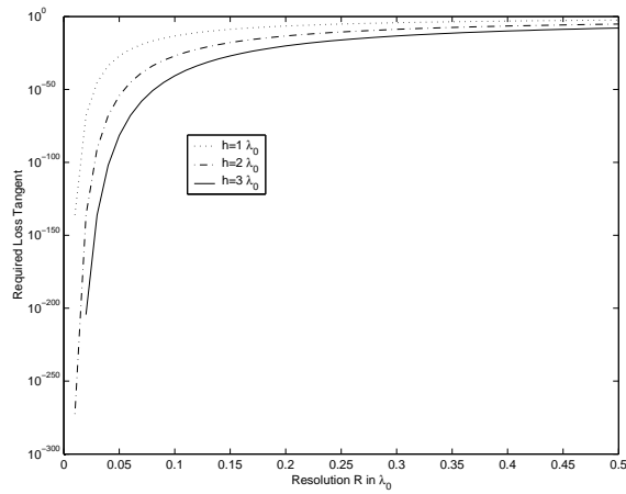
Figure 17: Required loss tangent of the LHM slab versus resolution in wavelength for different slab thicknesses.
