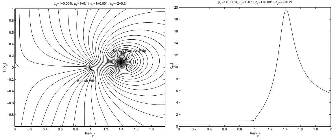
Figure 6: (Left) The contour plot of the magnitude of the reflection coefficient for a single negative material for the lower half space. A pole corresponding to the surface plasmon mode is observed. A branch point is on the real axis while the other branch point is on the imaginary axis [p. 100] [24]. (Right) Plot of the reflection coefficient magnitude along the real axis showing peaking near the pole. Here, \omega = \mu_0 = \epsilon_0 = 1 .
