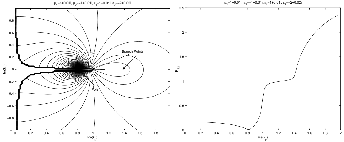
Figure 7: (Left) The contour plot of the magnitude of the reflection coefficient for an unmatched double negative material for the lower half space. Two poles are observed. (Right) Reflection coefficient plot along the real axis shows no large values along the real axis. Here, \omega = \mu_0 = \epsilon_0 = 1 .
