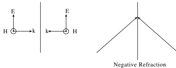
Figure 2: Negative refraction at an RHM/LHM interface is entirely due to the backward wave nature of one of the media, and is not a property restricted to LHM.
