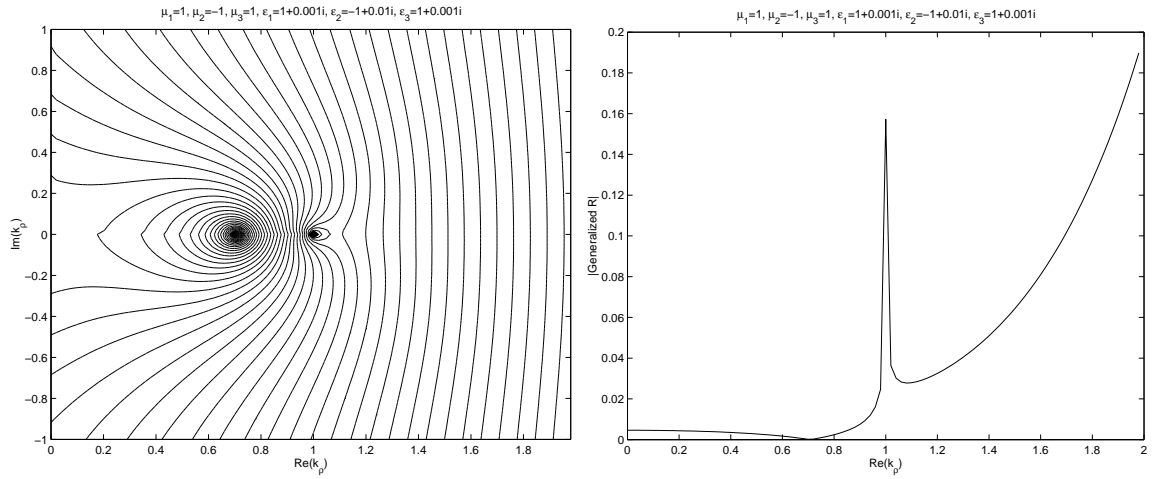
Figure 15: The contour plot of the magnitude of the LHM slab reflection coefficient (left) and the same coefficient along the real axis (right). Here, \omega = \mu_0 = \epsilon_0 = h = 1 .
