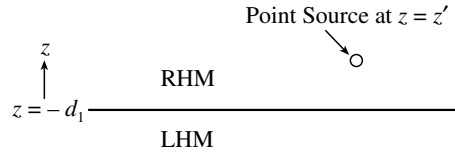
Figure 3: A point source over an LHM half space. The point source is located in the upper half space which is an RHM.
