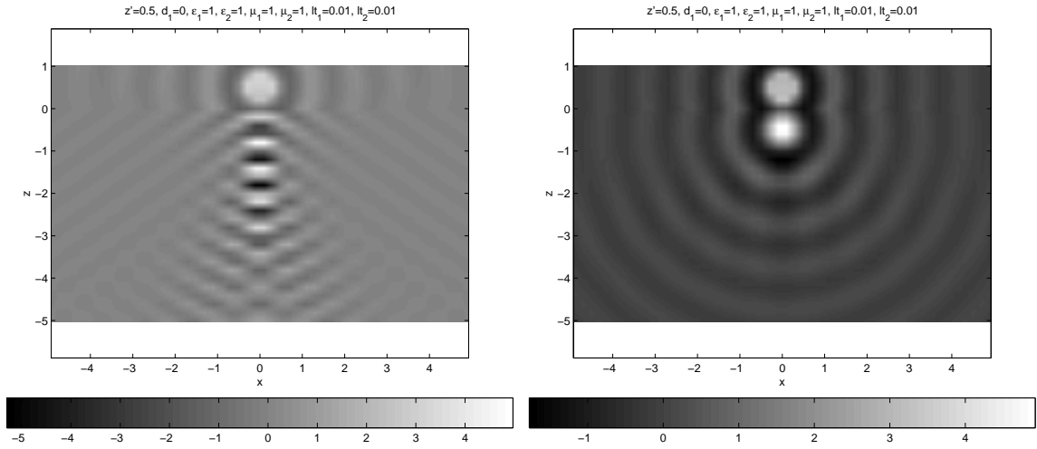
Figure 12: A point source above an LHM half space. (Left) The unmatched case gives rise to unfocussed wave along a caustic. (Right) The matched case gives rise to a partially focussed wave as the evanescent spectrum is not “time-reversed” even though the propagating spectrum is “time-reversed”. Dimensions are in free-space wavelength.
