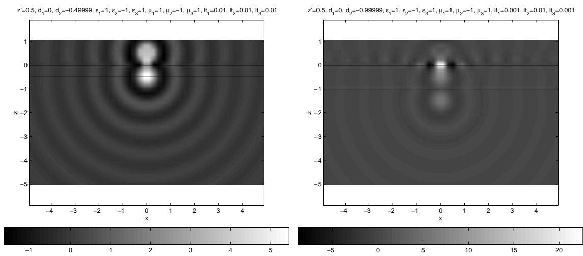
Figure 18: Contour plot of a snap shot of the field magnitude for a point source above an LHM slab. The source is placed at (\rho, z) = (0., 0.5) above the slab. The LHM slab is matched and has a thickness of 0.5 (left) and 1.0 (right). Dimensions are in wavelength. The source field is clipped at 3 to emphasize the other field.
